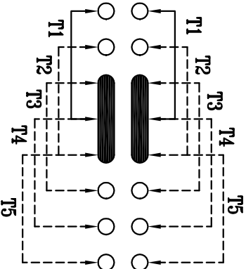
SCHEMATIC (SHORTING)
