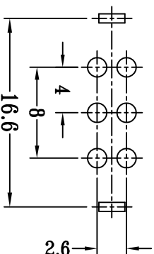
P.C.B LAYOUT BOTTOM VIEW
