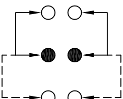
SCHEMATIC (NON-SHORTING)
