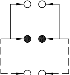
SCHEMATIC (NON-SHORTING)
