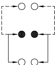
SCHEMATIC (NON-SHORTING)
