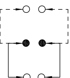
SCHEMATIC (NON-SHORTING)
