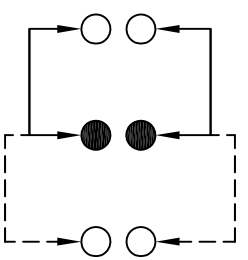
SCHMATIC (NON-SHORTING)
