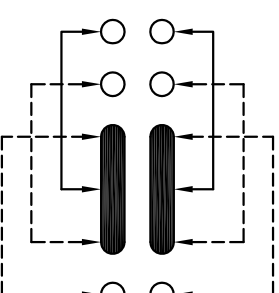
SCHEMATIC (NON-SHORTING)
