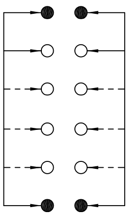
SCHMATIC (NON-SHORTING)
