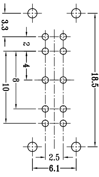
P.C.B LAYOUT BOTTOM VIEW
