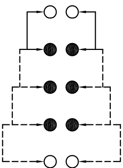
SCHEMATIC (NON-SHORTING)
