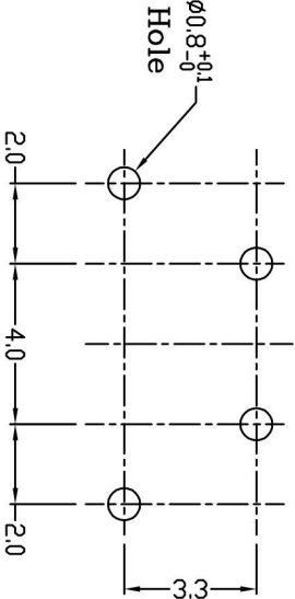
P.C. BOARD LAYOUT BOTTOM VIEW
