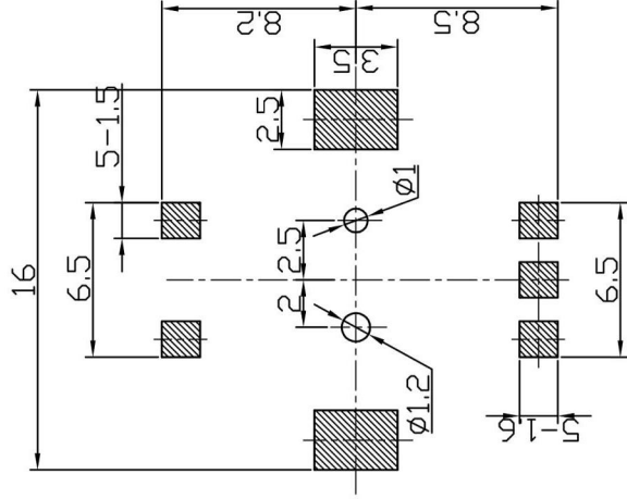
P.C.BOARD MOUNTING HOLE DIMENSIONS
