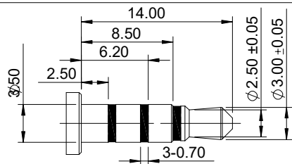
PLUG SPEC
