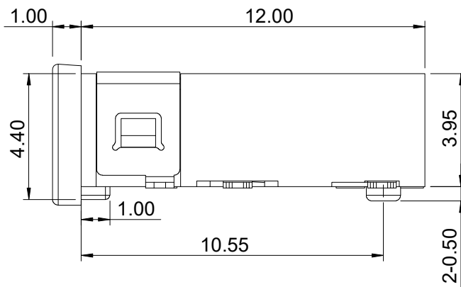
3.50mm 4 POLE PLUG DETAIL DRAWING(2:1)
