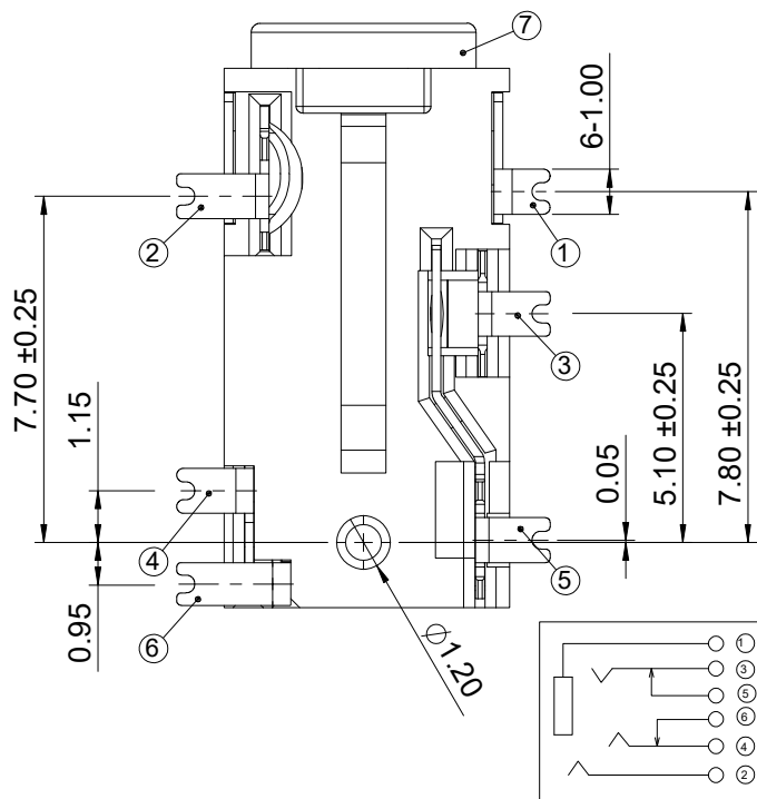
SCHEMATIC
