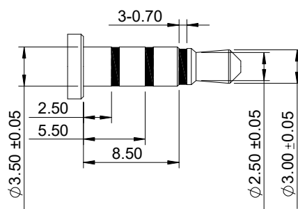
3.50mm 4 POLE PLUG DETAIL DRAWING(2:1)
