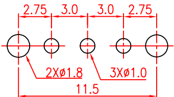
P.C.B LAYOUT TOP VIEW
