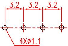
P.C.B LAYOUT TOP VIEW
