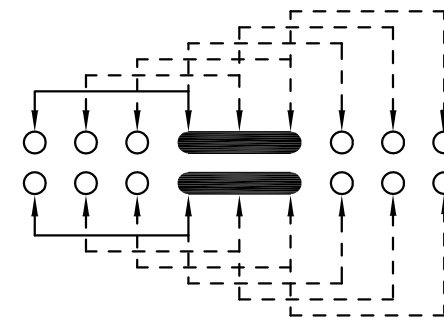
SCHEMATIC (SHORTING)
