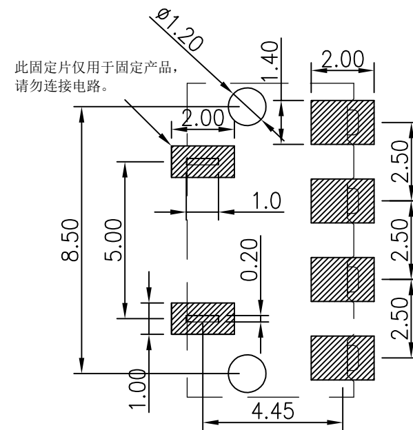
RECOMMENDED PCB LAYOUT TOP VIEW (.XX±0.05)
