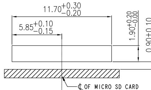
RECOMMEND ID DIMENSION
