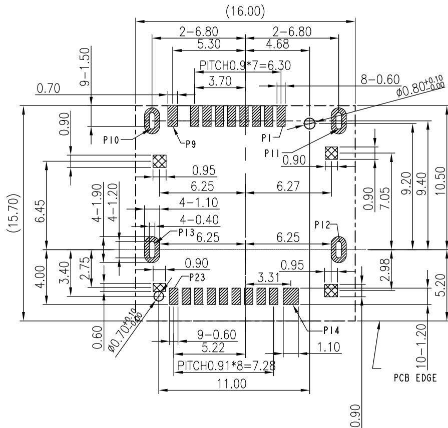
Recommended P.C.B LAYOUT TOP VIEW (TOLERANCE \pm 0.05 )
