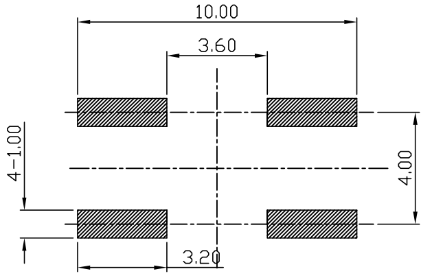
SOLDER LAND DIMENSION
