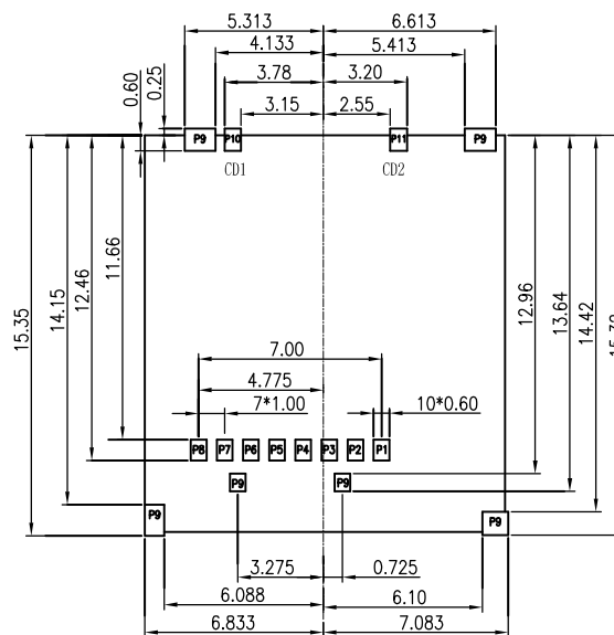
PCB LAYOUT
