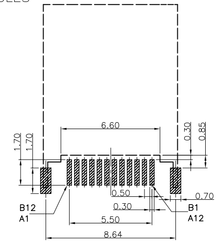
RECOMMENDED P.C.B. LAYOUT (T:0.8mm)
