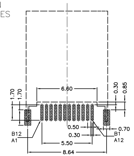
RECOMMENDED P.C.B. LAYOUT (T:0.8mm)
