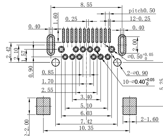
RECOMMENDED PCB LAYOUT (TOP VIEW) DEFAULT TOLERANCE: ±0.05
