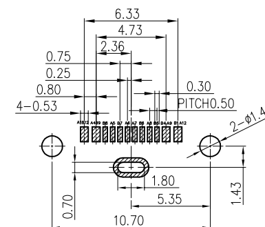
RECOMMENDED P. C. B LAYOUT TOP VIEW (TOLRANCE:±0.05)
