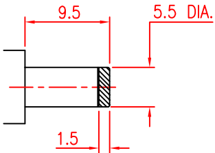
MATE PLUG
