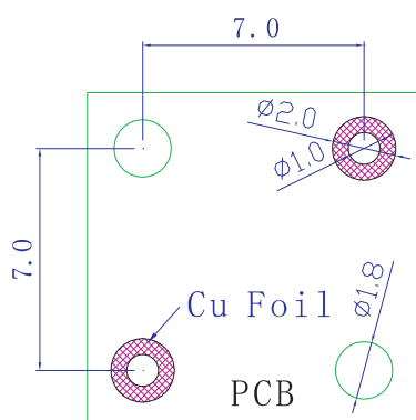
PCB Hole Layout
