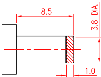
MATE PLUG
