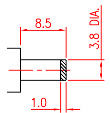
MATE PLUG
