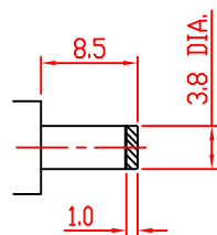
MATE PLUG
