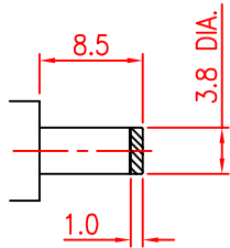
MATE PLUG
