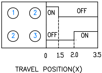
SWITCHING SEQUENCE
