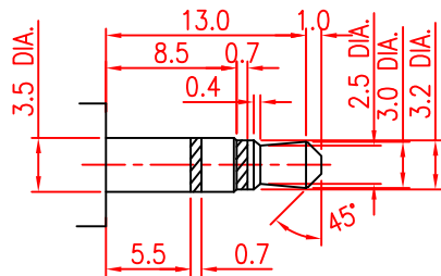
MATE PLUG
