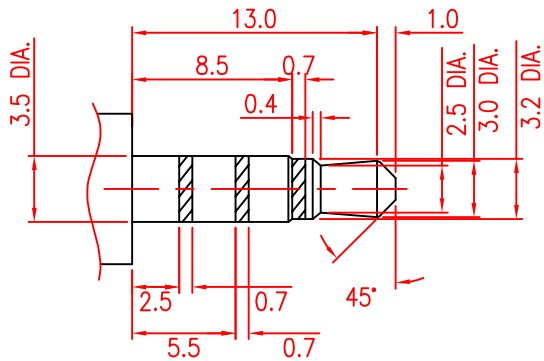
MATE PLUG
