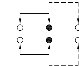
SCHEMATIC (NON-SHORTING)
