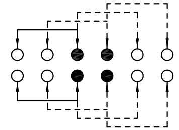
SCHEMATIC (SHORTING)
