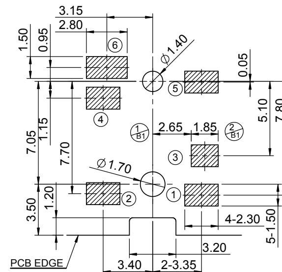
RECOMMENDED PCB LAYOUT(TOP VIEW) (GENERAL TOLERANCE \pm 0.05 )
