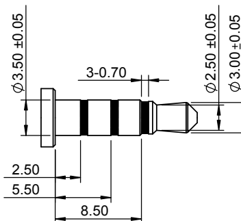
Ø 3.50mm 4 POLE PLUG DETAIL DRAWING(2:1)
