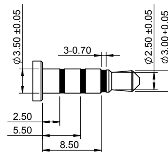
Ø3.50mm 4 POLE PLUG DETAIL DRAWING(2:1)
