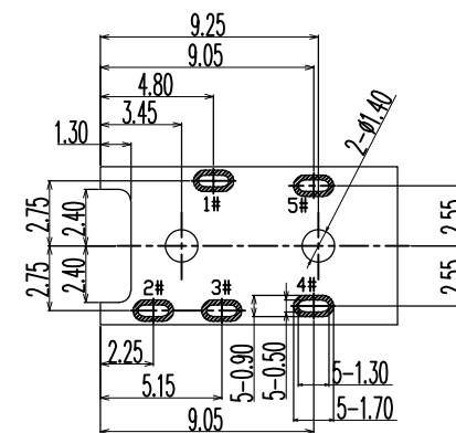
P.C.B LAYOUT T=1.00mm TOP VIEW
