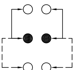
SCHEMATIC (NON-SHORTING)
