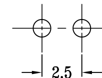
P.C.B LAYOUT BOTTOM VIEW
