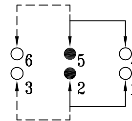
SCHEMATIC (NON-SHORTING)
