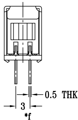
VIEW K
