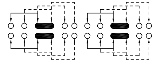
SCHEMATIC (SHORTING)
