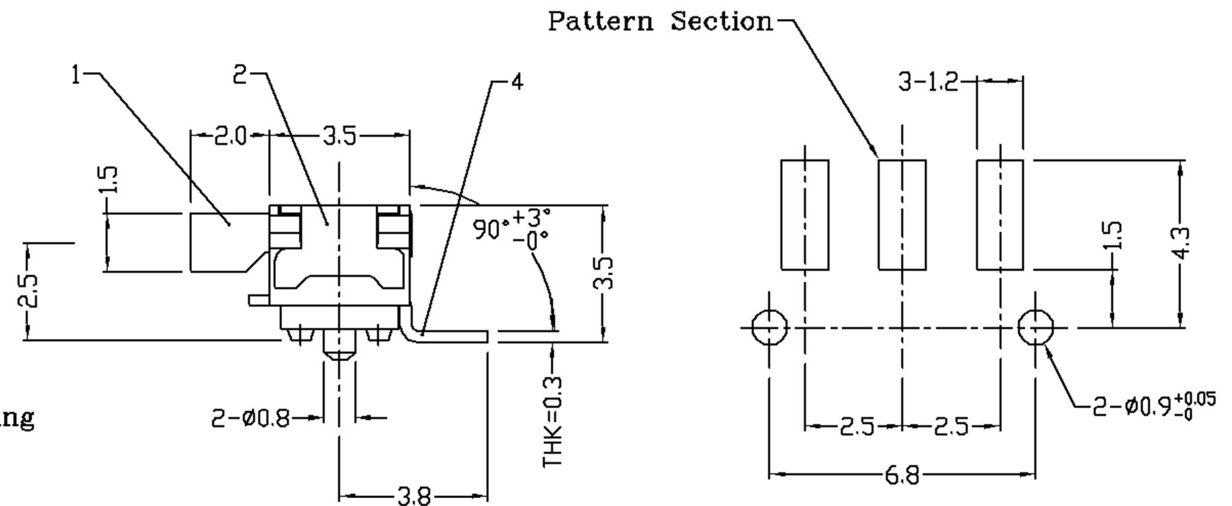
P.C. BOARD LAYOUT
