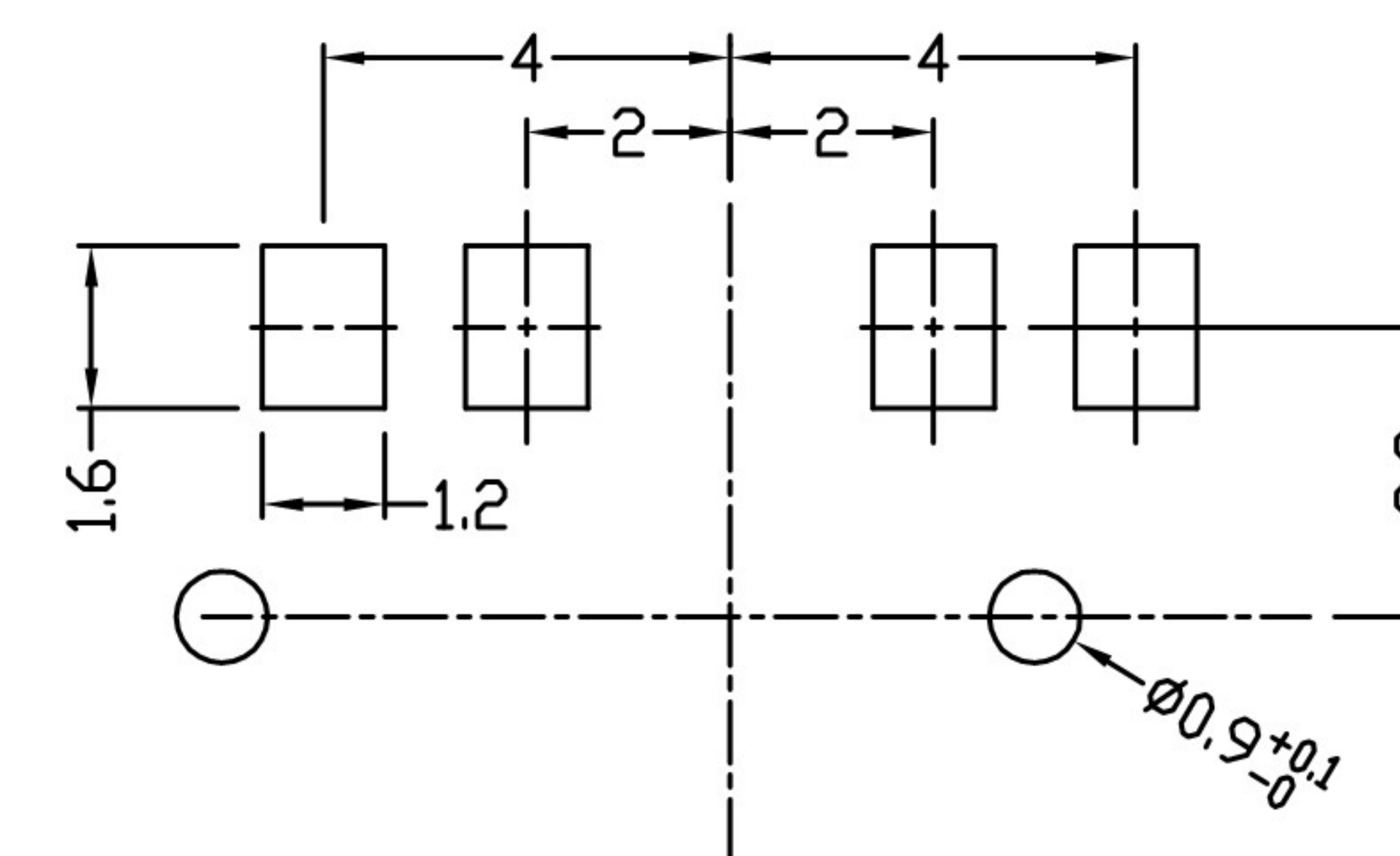
P.C. BOARD LAYOUT BOTTOM VIEW
