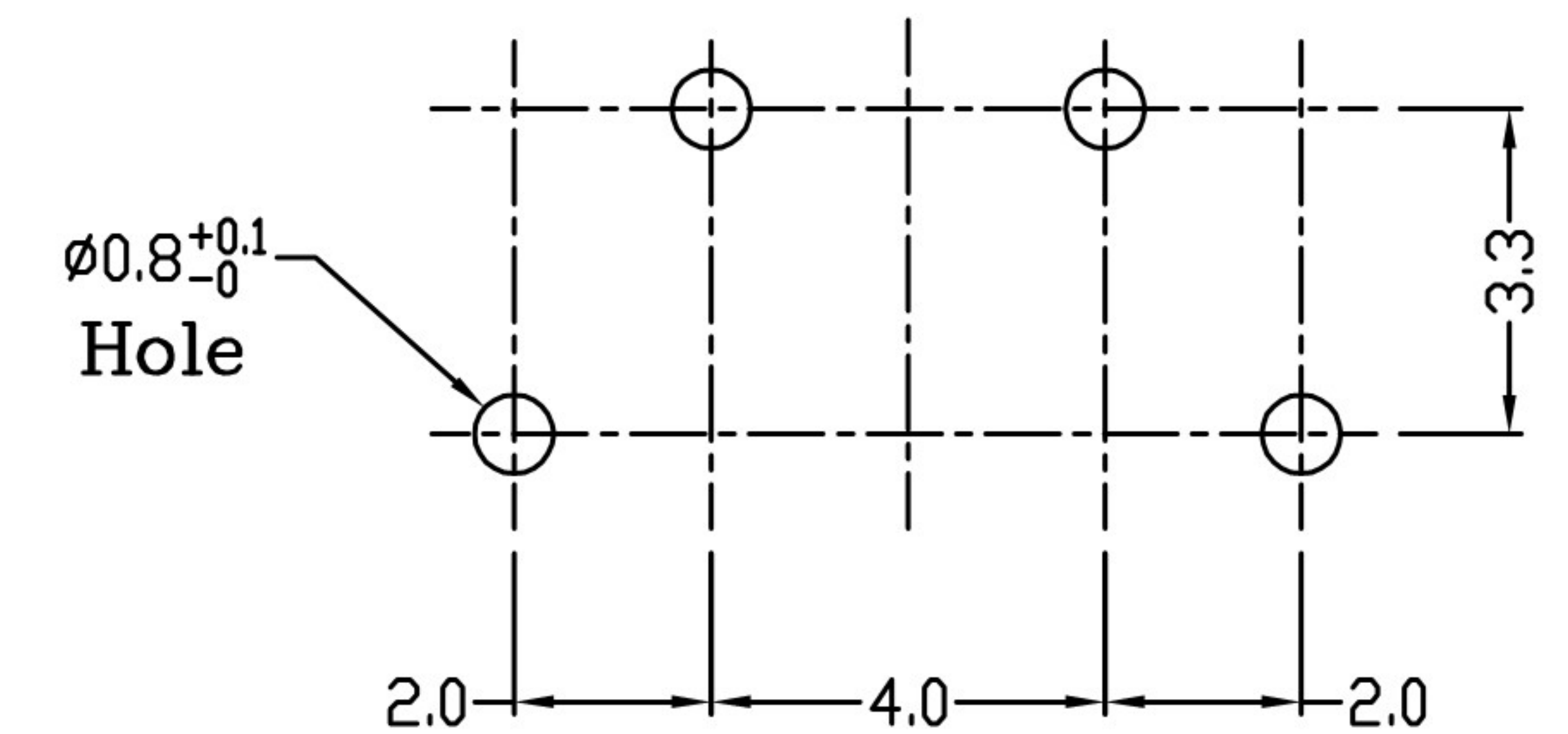
P.C. BOARD LAYOUT BOTTOM VIEW
