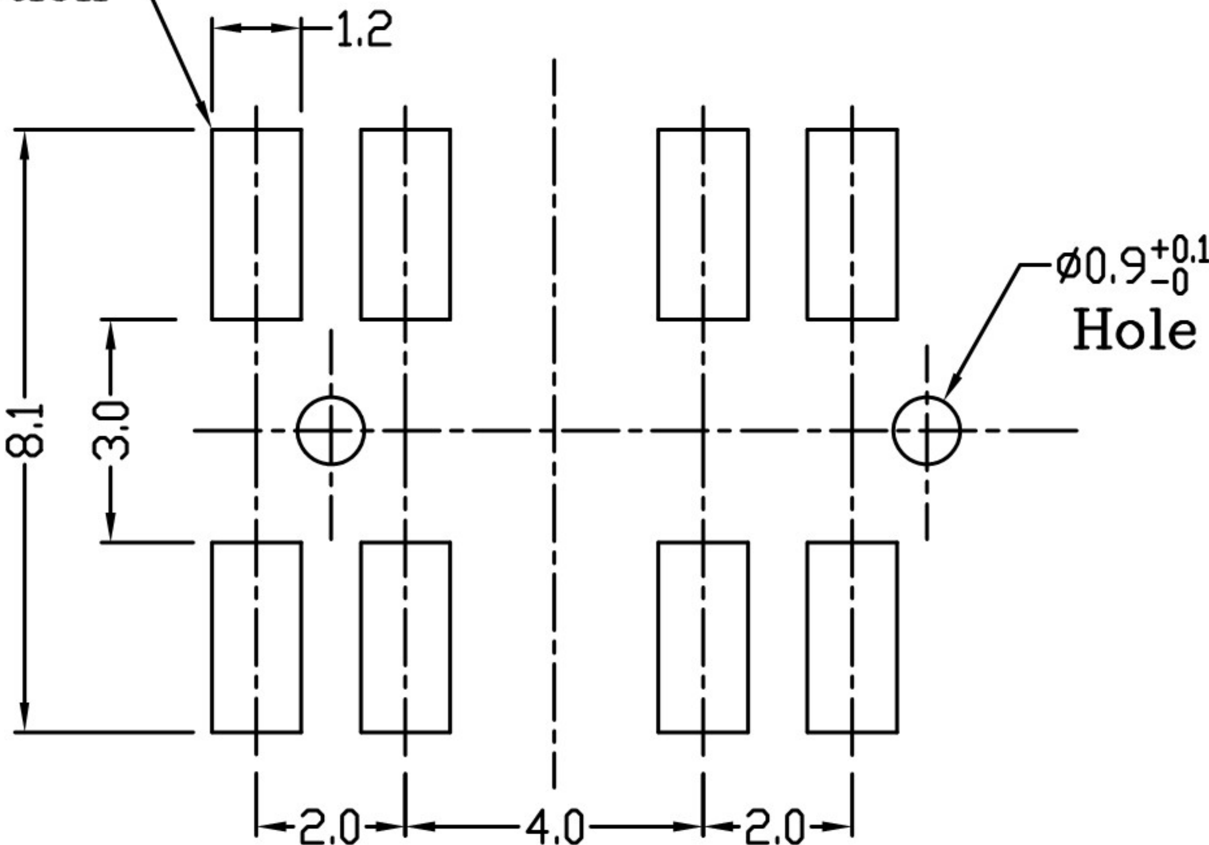
P.C. BOARD LAYOUT BOTTOM VIEW
