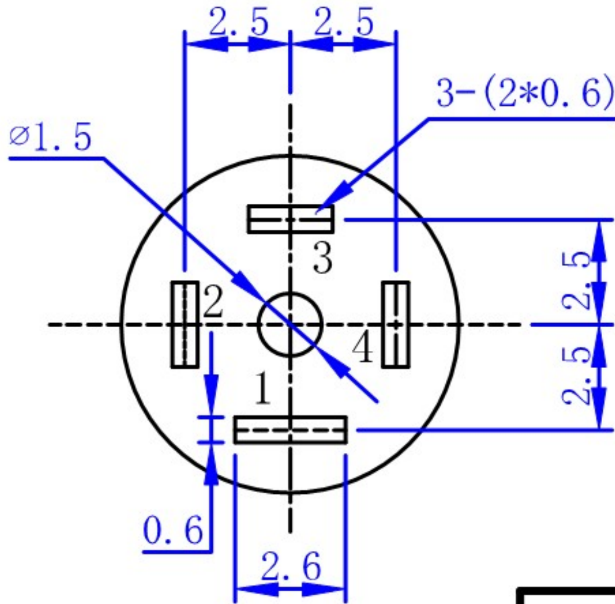
P. C. B. LAYOUT TOP VIEW
