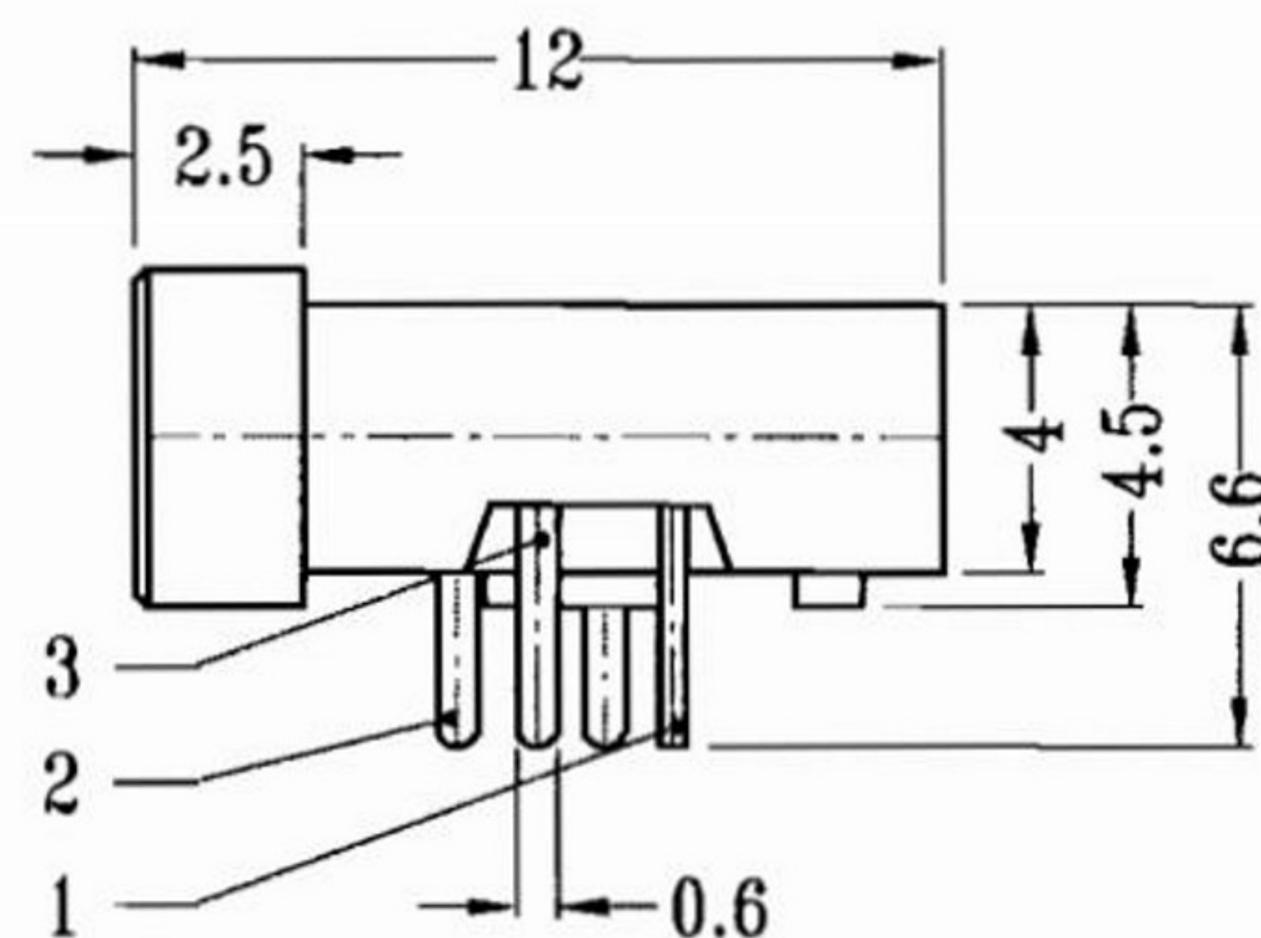
SCHEMATIC ST-103-C-03
