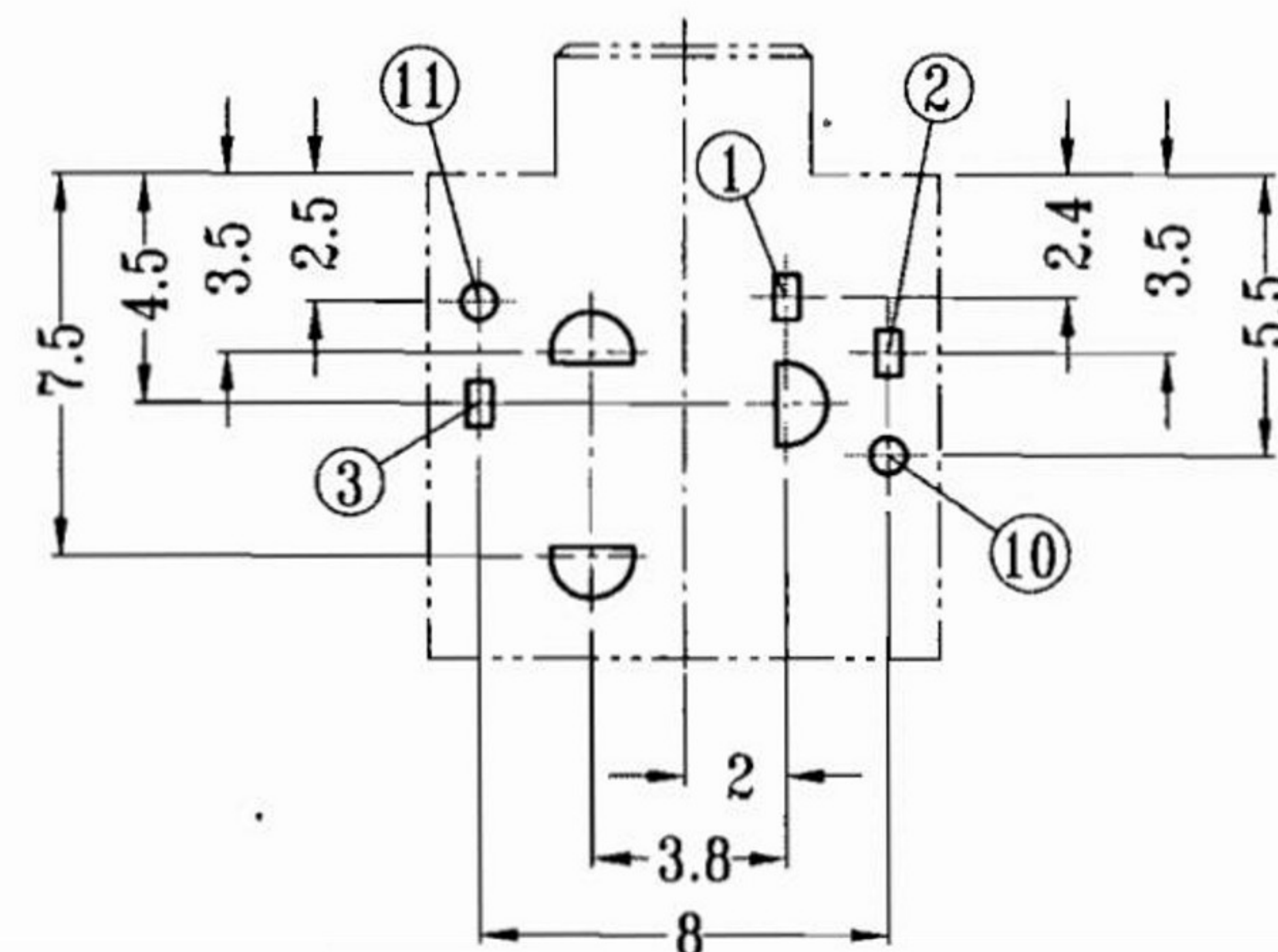
P.C.B LAYOUT BOTTOM VIEW
